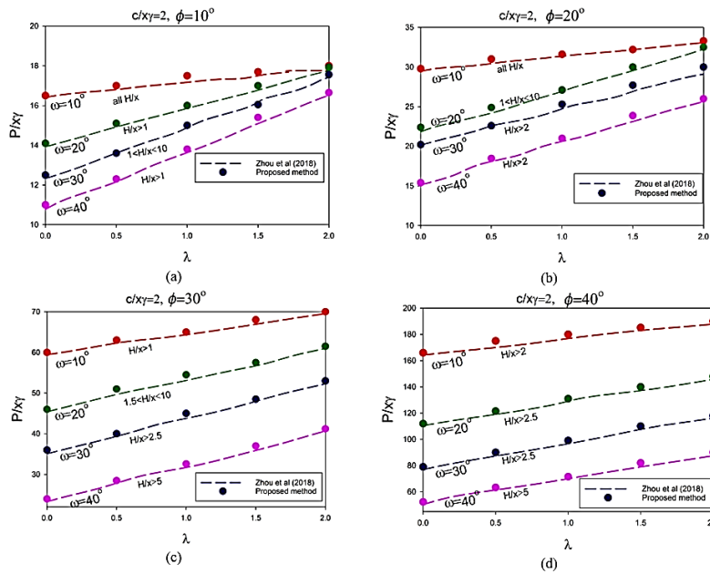
Fig. 6: Variation of P/xy with \lambda for different slope's angle and normalized slope's height and c/xy=2 (a) \phi=10^\circ (b) \phi=20^\circ (c) \phi=30^\circ (d) \phi=40^\circ
