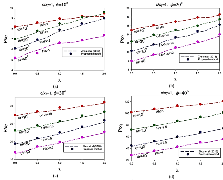
Fig. 5: Variation of P/xy with \lambda for different slope's angle and normalized slope's height and c/xy=1 (a) \phi=10^\circ (b) \phi=20^\circ (c) \phi=30^\circ (d) \phi=40^\circ
