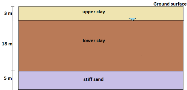
Figure 2. Soil profile showing different layers.
