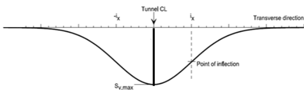
Figure 1. Gaussian curve for transverse surface settlement trough.
