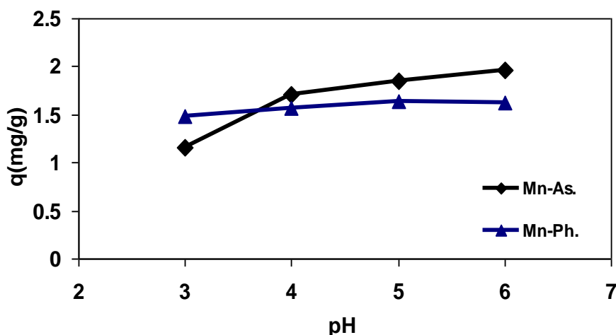
Figure 4: Effect of pH on Mn biosorption on A. Niger and Ph. Chrysosporium
