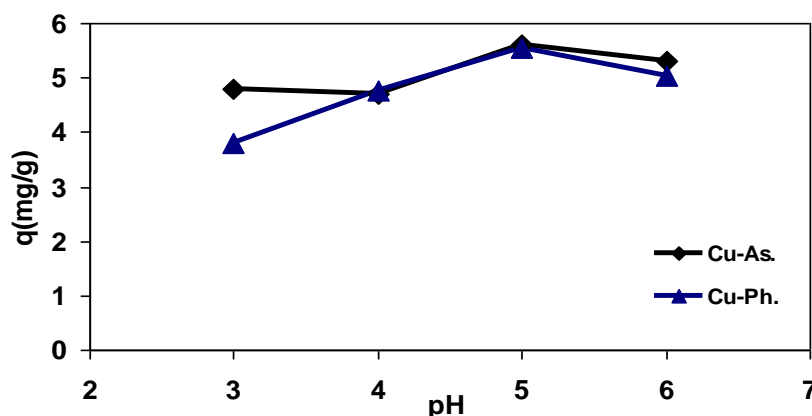
Figure 3: Effect of pH on Cu biosorption on A. Niger and Ph. Chrysosporium
