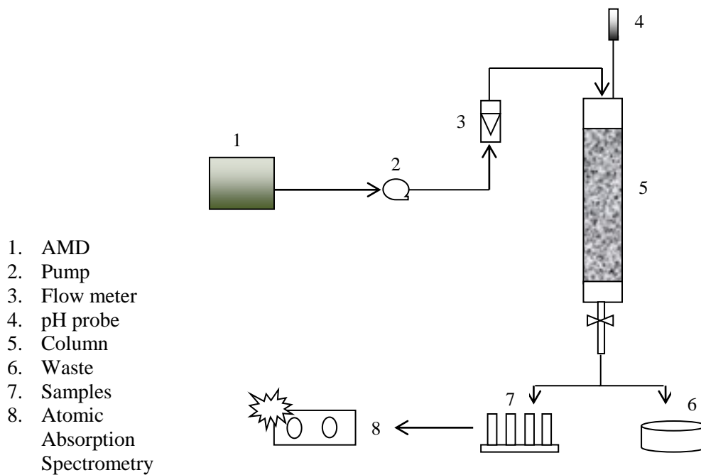
Figure 2: Experimental Set-up
