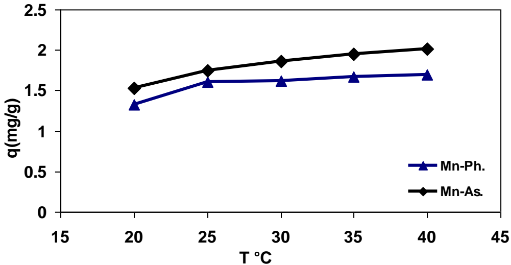
Figure 8: Effect of temperature on Mn biosorption on A.Nniger and Ph. Chrysosporium
