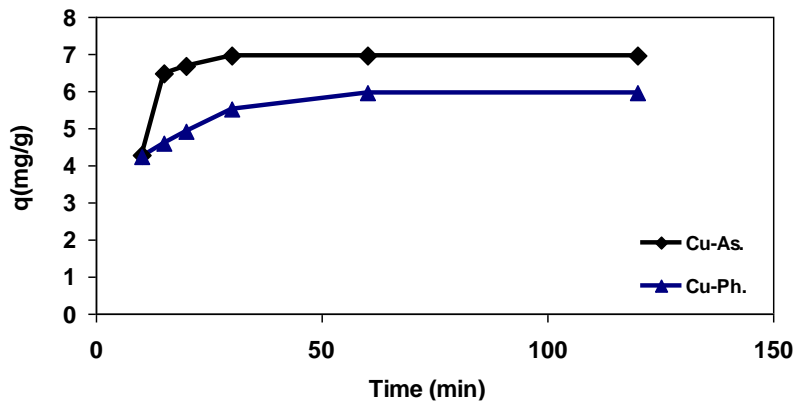
Figure 5: Effect of contact time on Cu biosorption on A. Niger and Ph. Chrysosporium
