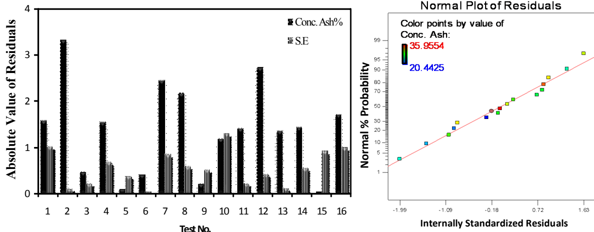
Figure 4: Normal graphs of residual values (right), residual values of responses from performed tests and obtained results from model for non ground sample in 16 performed tests (left)
