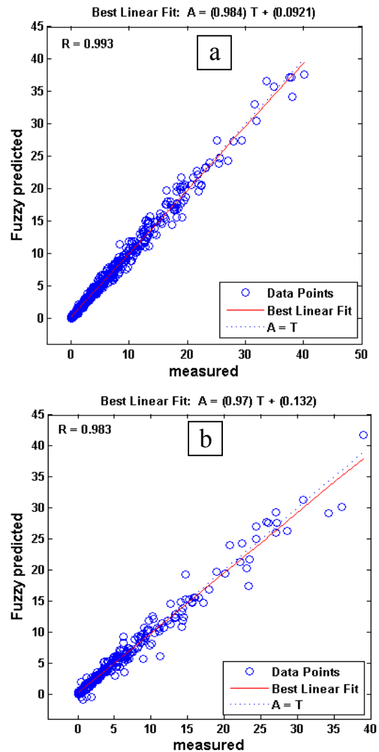
Figure 10: Correlation between measured values in laboratory and predicted values by neuro-Fuzzy model for training (a) and test data (b).
