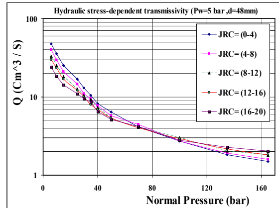
Figure 6: Three stages of joint roughness effect on stress dependent hydraulic transmissivity in 48 mm diameter and 5 bars water pressure
