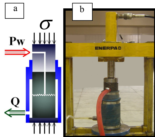
Figure 1: a) Schematic of the jointed rock sample surrounded by a cover subjected to the axial load b) The picture of the laboratory setup
