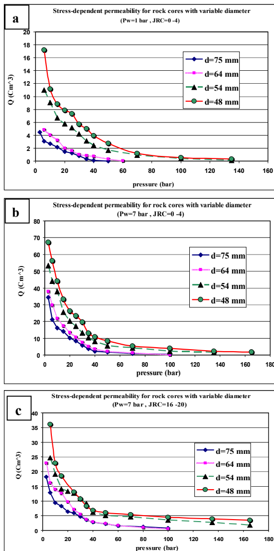
Figure 3: Volume of passed water as a function of normal stress for different joint roughness
