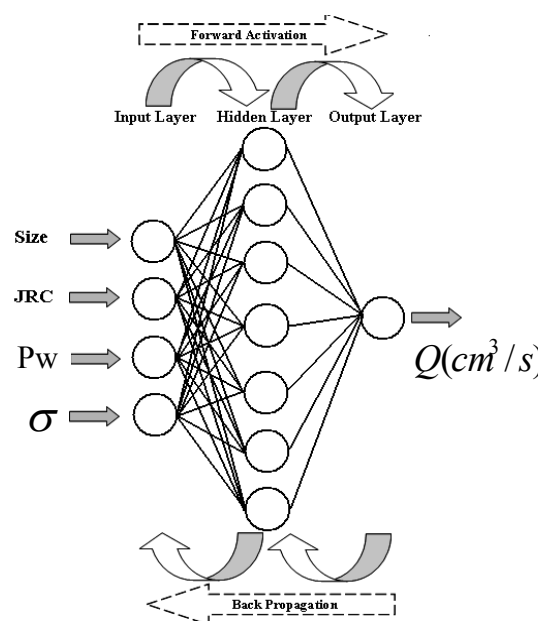
Figure 7: Back propagation neural network used for flow rate estimation
