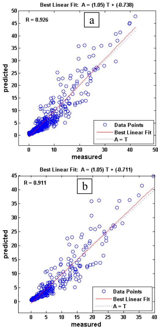
Figure 12: Correlation between measured values in lab and predicted values by regression for data set using in determined of unknown coefficient (a) and new data (b).
