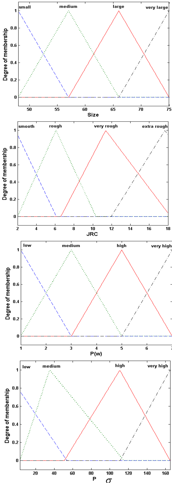
Figure 9: Membership function for input parameters after training by neural network
