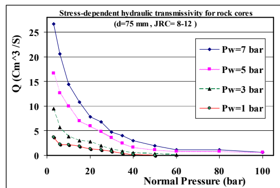
Figure 4: Effect of water pressure variation on stress dependent transmissivity in 48 mm diameter and roughness coefficient between 8 and 12
