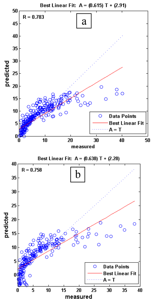
Figure 11: Correlation between measured values in lab and predicted values by regression for data set using in determined of unknown coefficient (a) and new data (b)
