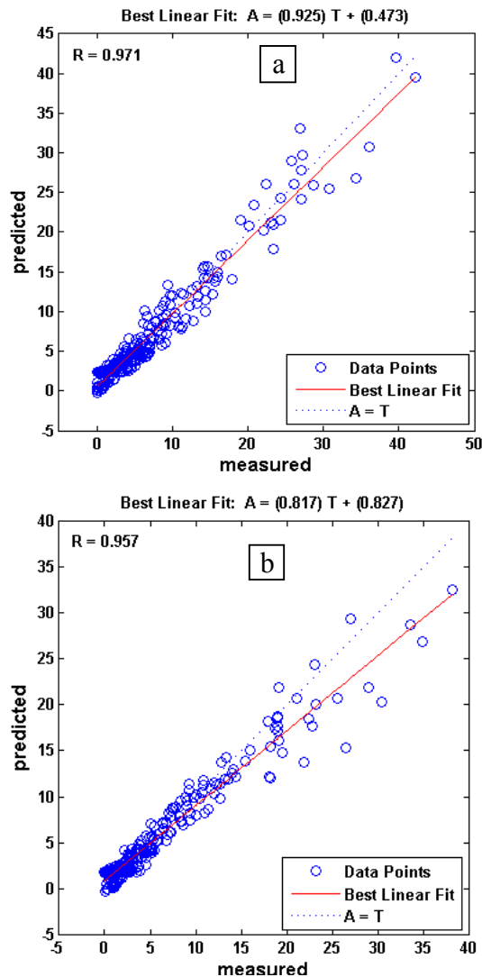
Figure 8: Correlation between measured and predicted values for training (a) and test data(b)
