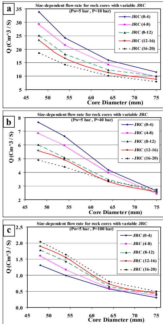
Figure 5: Effect of joint roughness on water flow rate versus diameter in 5 bars water pressure under a) low, b) medium and c) high stress condition
